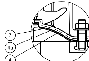
PTFE diaphragm with cushion cover.
